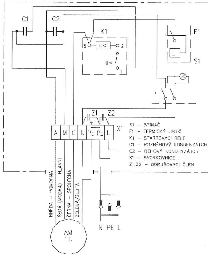
ELEKTROMOTOR 1PJ60390 01, 1,1kW, 230V, 50Hz
